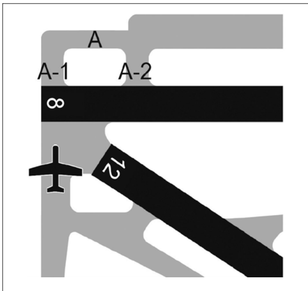
FIG 3-9-12 Runway/Taxiway Proximity
