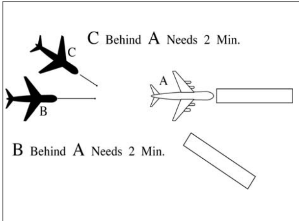
FIG 6-1-3 Arrival Minima
